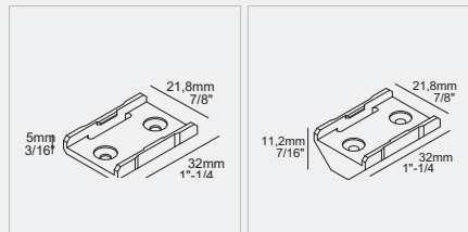
SHL19-MOUNTING CLIP
